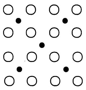
3D bonding
