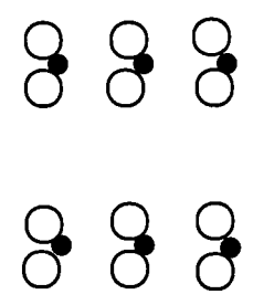
molecular
